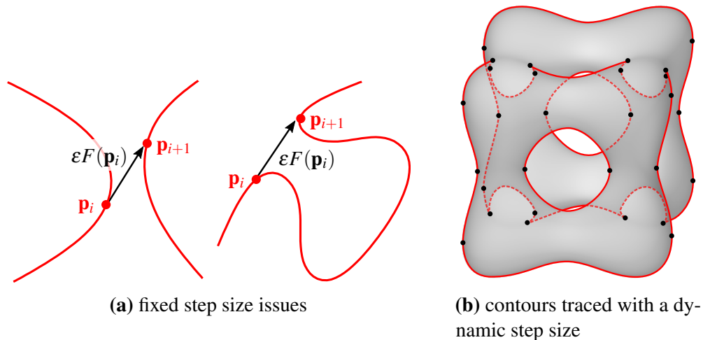
Figure 8.2: Implicit surface contour generator tracing — With a fixed step size (a), the traced contour may jump to another component of the contour (left) or skip a part of it (right). (b) With a dynamic step size integration scheme, Plantinga and Vegter (2006) accurately trace the contour generator of a complex implicit tangle cube: x^4 - 5x^2 + y^4 - 5y^2 + z^4 - 5z^2 + 10 = 0 . The starting points are indicated by the black dots.
