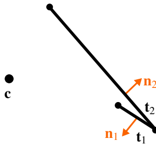
Figure B.3: Counterexample for Markosian's definition of front/back-facing edges — In this example, the face nearest to the camera is t_2 , which is back-facing. Therefore the contour edge between the triangles would be marked as back-facing and thus invisible. In fact, t_1 occludes t_2 , even though t_2 is nearer to the camera. This is a convex edge, and thus potentially visible.
